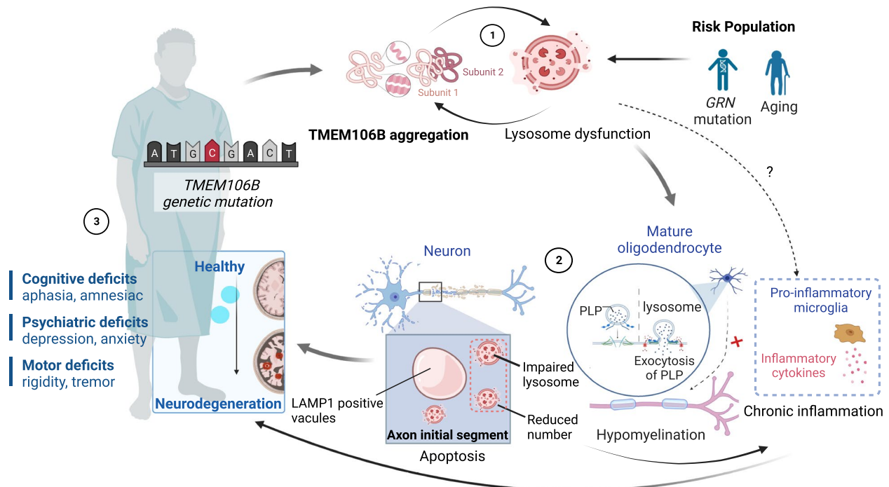
Fig. 4 Overall description of TMEM106B related disease pathology. TMEM106B and lysosome dysfunction forms a vicious cycle. TMEM106B deficiency triggers abnormal lysosome manifestations in neuron: reduced number, abnormal localization at the axon initial segment or perinuclear space and a vacuole-like shape. TMEM106B abnormal aggregation also induces hypomyelination by oligodendrocyte, further activating microglia-related neuroinflammation, disrupting signal transduction and related physiological process and driving the cognitive, psychiatric, and motor lesions in diverse neurodegenerative diseases. Other risk factors like aging or GRN mutation also contribute to this cycle via affecting lysosome functions
