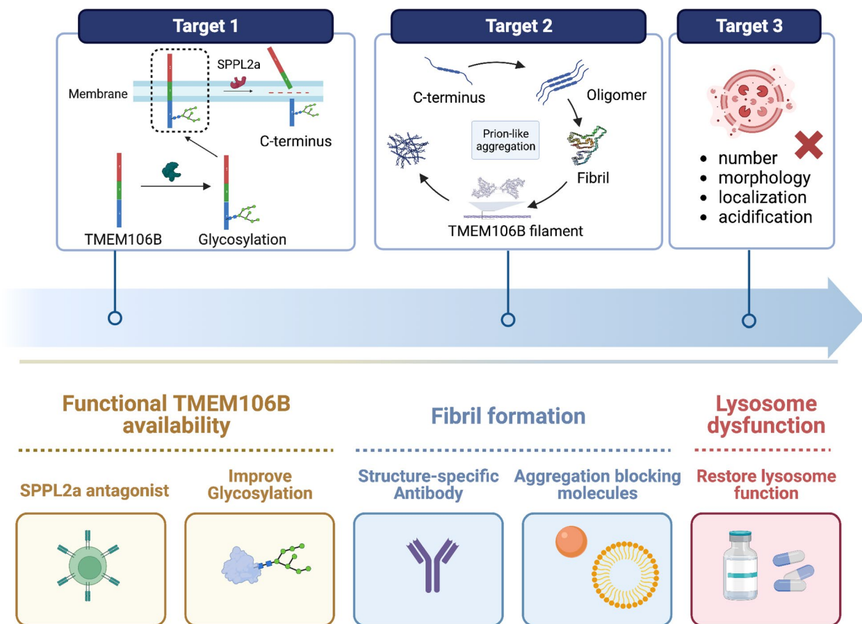
Fig. 5 Multiple therapeutic strategies targeting TMEM106B for intervention. We proposed that the formation of TMEM106B fibrils may be the key turning point that initiates the downstream pathogenic cascade. Several TMEM106B- or lysosome-based therapeutic approaches have been proposed, including inhibitors of cleavage, improvement of TMEM106B glycosylation, immunotherapy using antibodies against oligomer fibrils, C-terminus aggregation inhibitors and stabilization of lysosome
