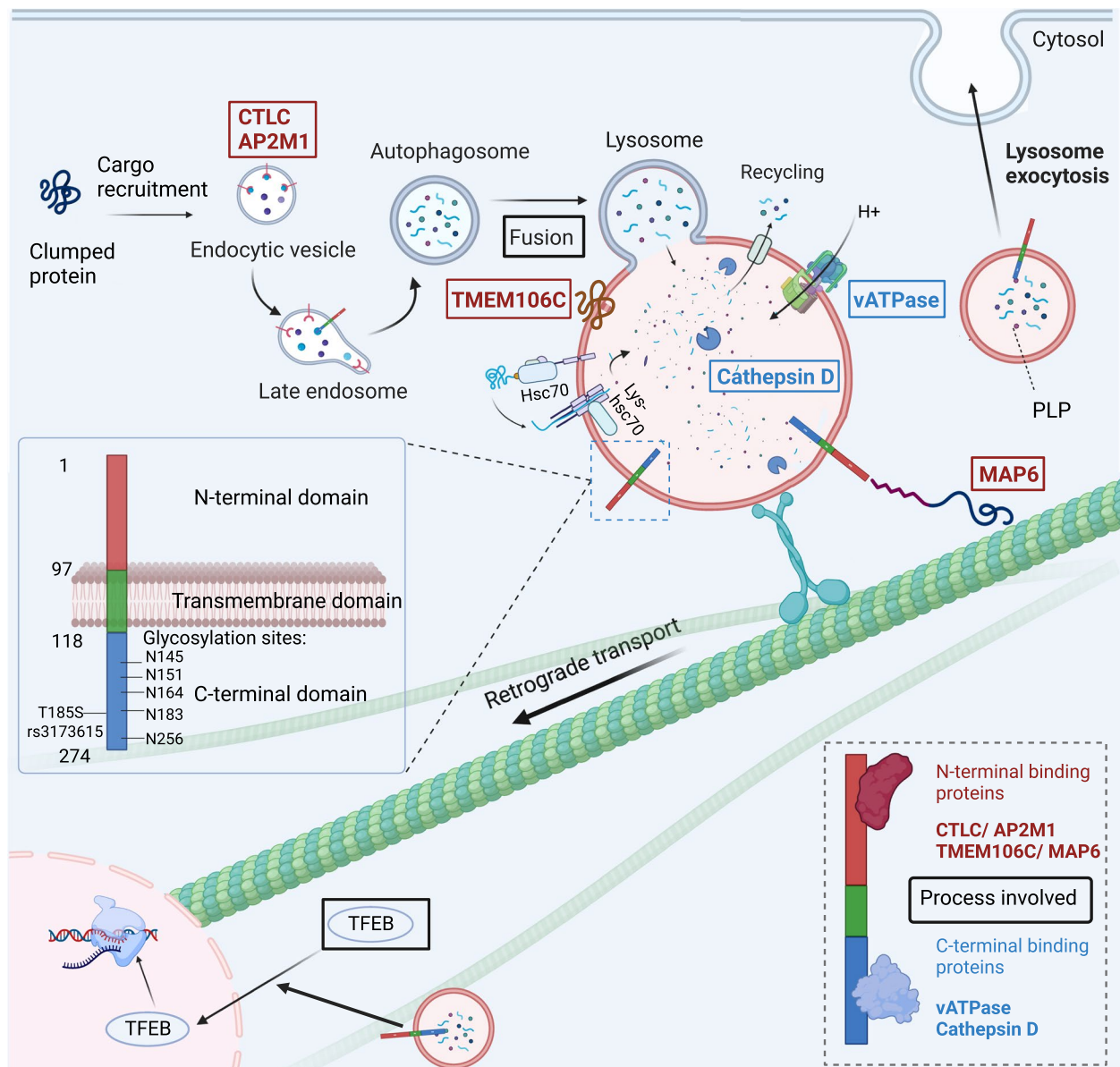
Fig. 2 The physiological roles of TMEM106B under healthy conditions. TMEM106B is a type II transmembrane protein located on late endosome and lysosome, which has 274 residues and three structural domains. This C-terminal fragment (118–274 residue) contains five important N-glycosylation sites (N145, N151, N164, N183, N256). Proteins with known interaction with N-terminal TMEM106B are circled in red and C-terminus in blue. TMEM106B interacts with AP1 and v-ATPase V0 domain subunits, which controls the acidification of lysosomes. The interaction with MAP6 regulates lysosome retrograde transport. TMEM106B further activates TFEB-dependent lysosome biogenesis. Lysosomal activity is significantly modulated by intraluminal pH in addition to enzyme concentration and lysosome location within the cell to correctly degrade the contents. Endosome and lysosome fusion is also mediated by TMEM106B. TMEM106B plays important roles in the transportation, maturation and biogenesis of lysosomes. TMEM106B regulates lysosome traffic and exocytosis to affect PLP to be transported to the myelin sheath in oligodendrocytes
